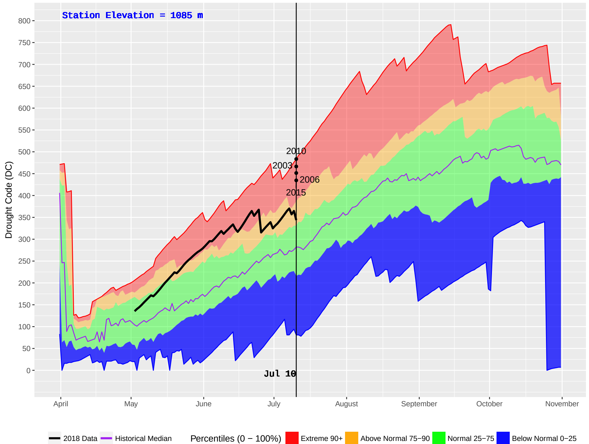
TAUTRI (206) : Historical (1970–2016) and Current (2018) Noon Drought Code (DC)
