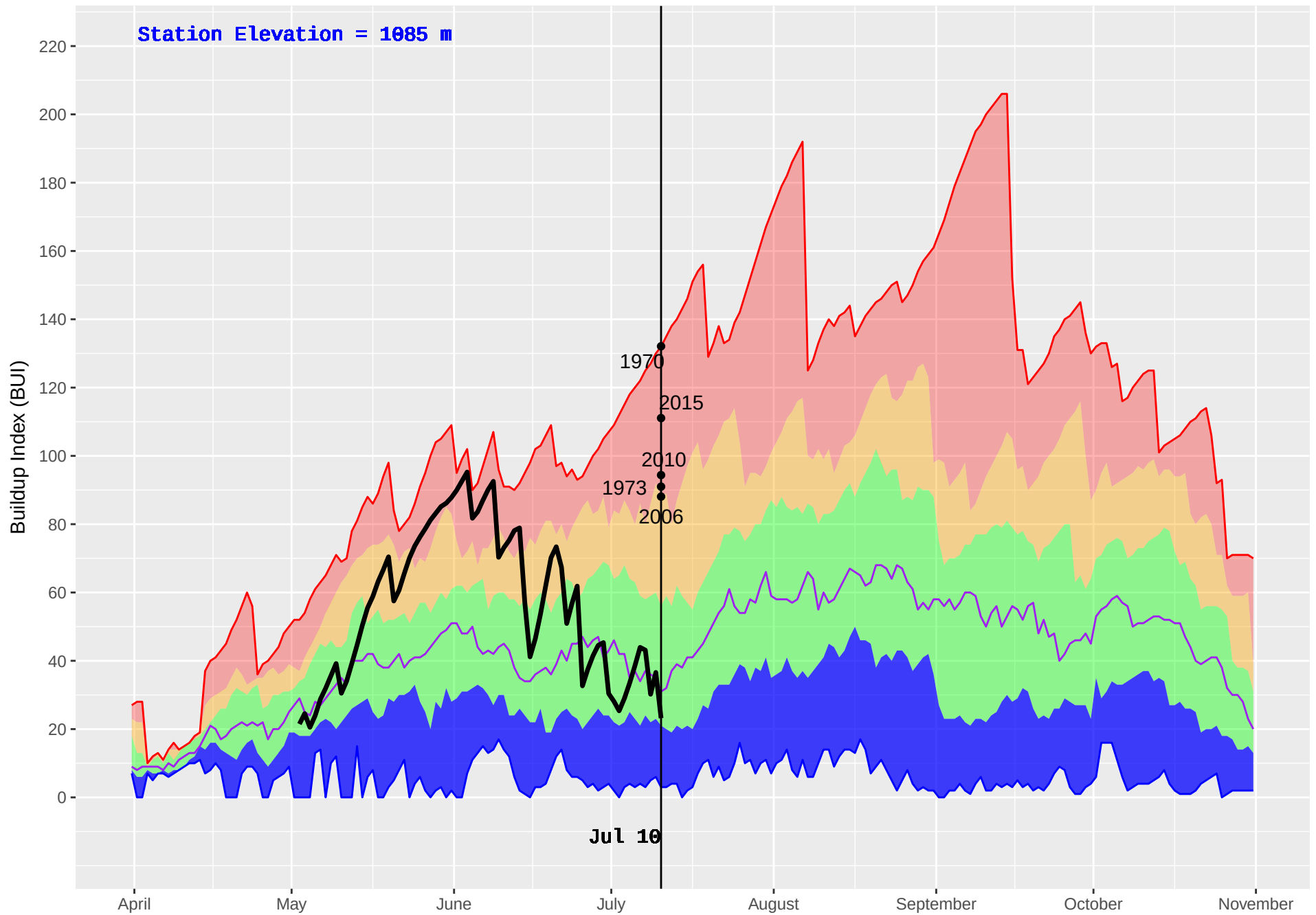
TAUTRI (206) : Historical (1970–2016) and Current (2018) Noon Buildup Index (BUI)
